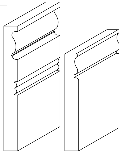
Victorian Plinth 5-1/2" x 9" x 1" Classic Plinth 3-1/2" x 7" x 1 4-3/4" x 9" x 1 5-1/2" x 9" x 1
